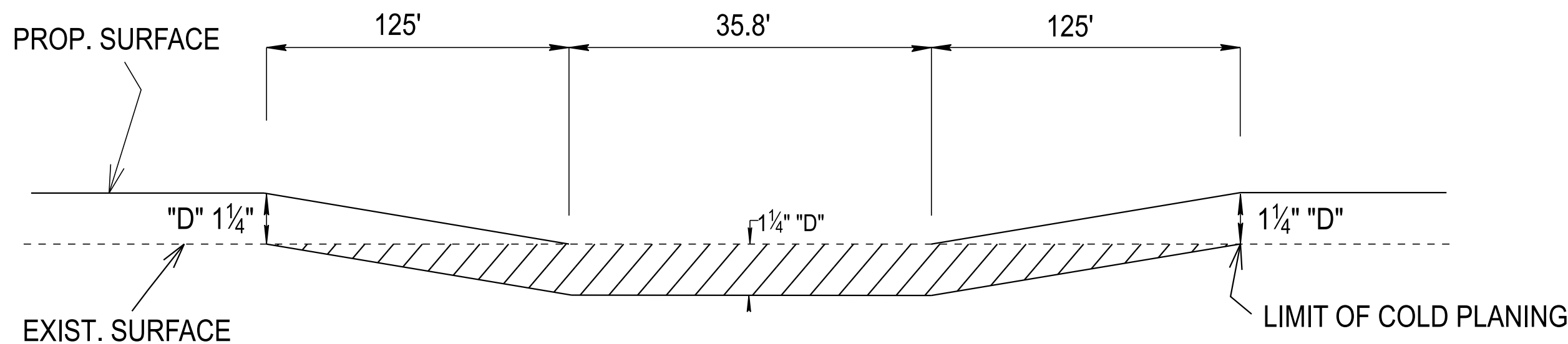
DETAIL OF RESURFACING TRANSITION FOR BRIDGE OVER TOWN CREEK AT L.M. 13.89
